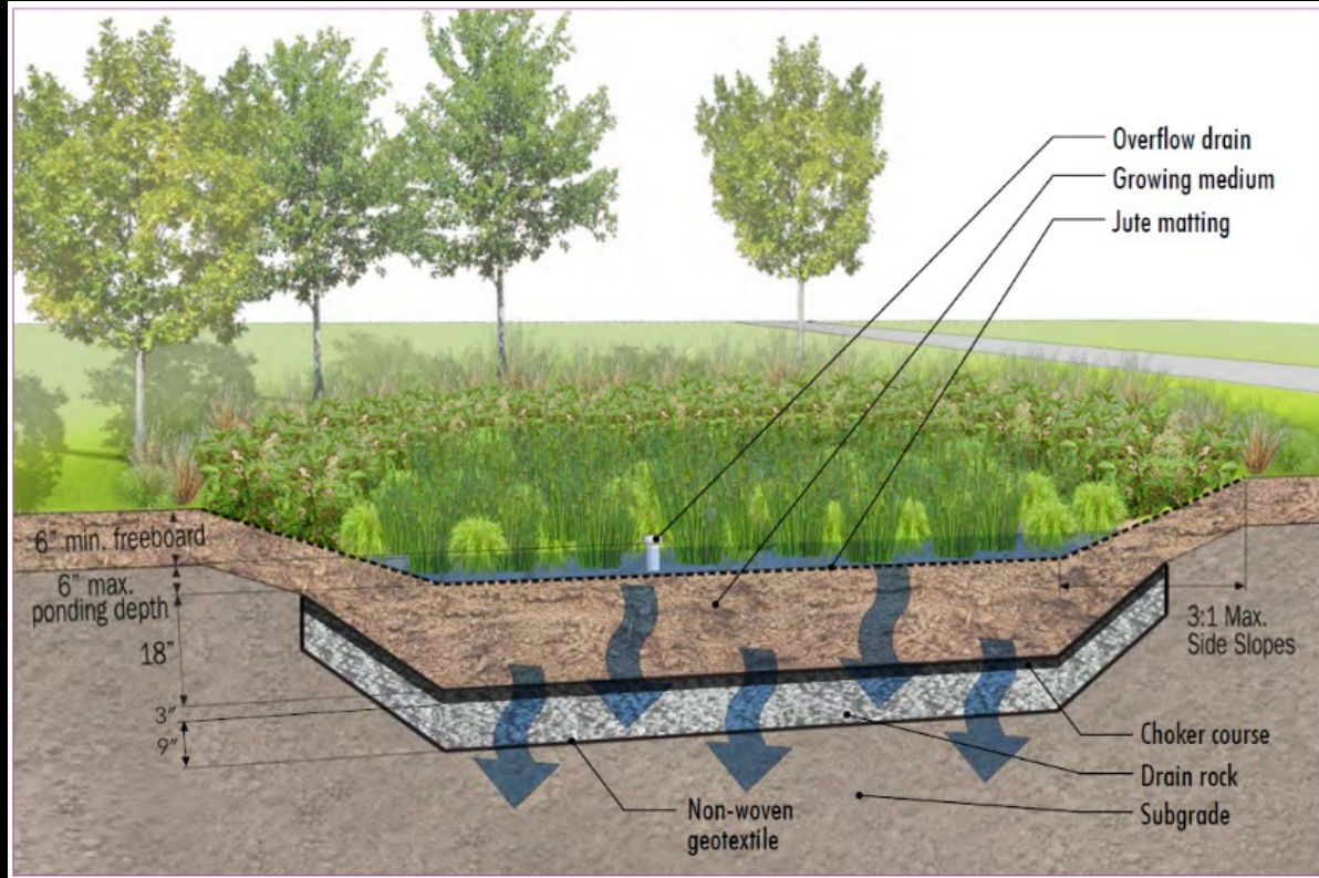
bioretention swale
